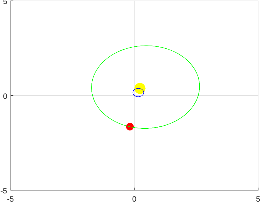
Celestial Mechanics: Two (2) Body Problem Problem 9 (RK4): m_1=0.03 , m_2=0.3 (fig01.fig)
